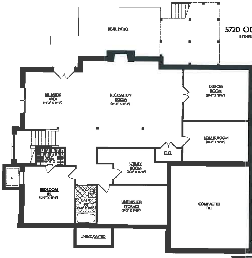
BASEMENT FLOOR PLAN AREA: 2,074 SQ FT
